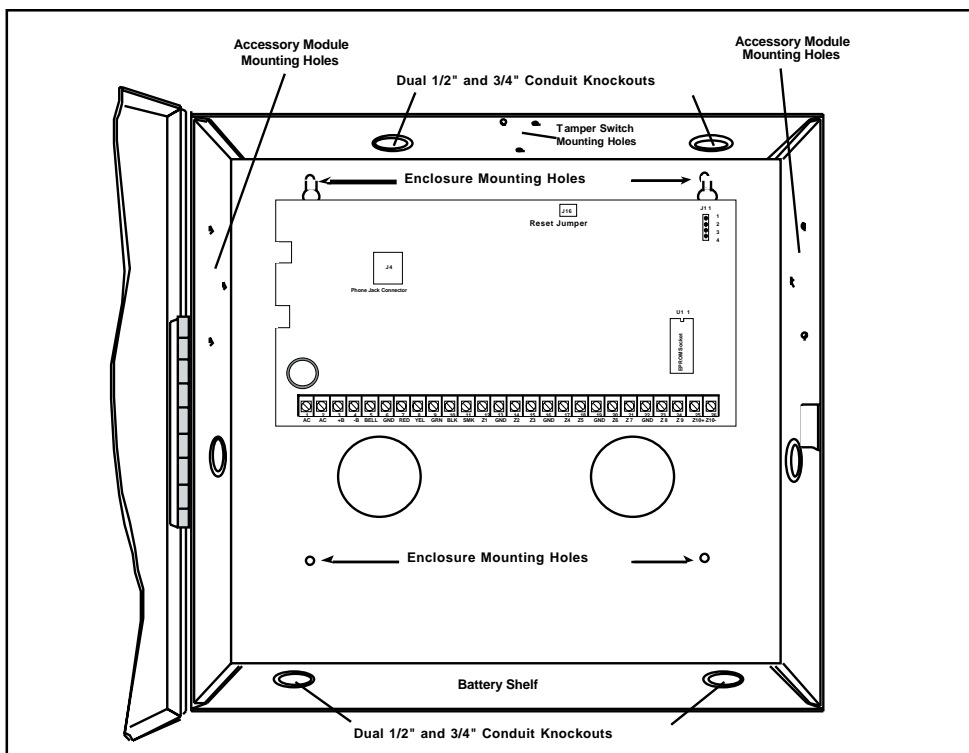
Figure 2A: XR6/XR10/XR20 in optional 349 Enclosure
