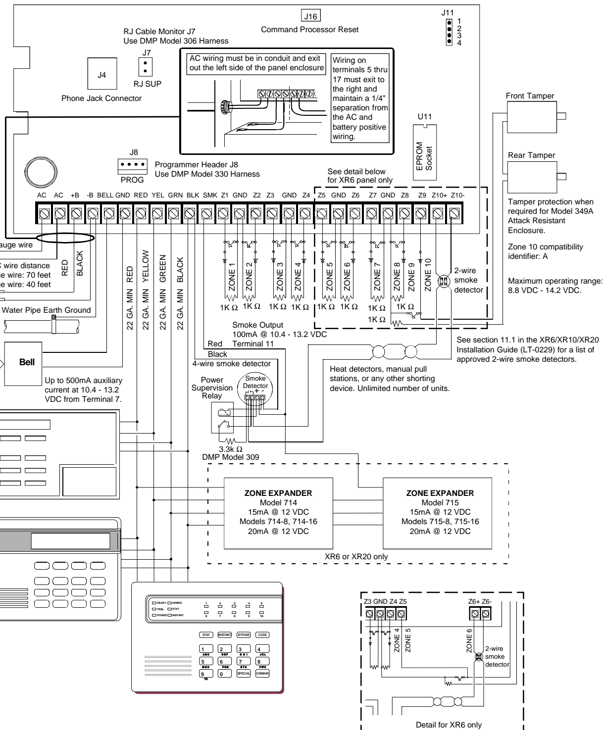
Figure 1: XR6/XR10/XR20 wiring diagram
