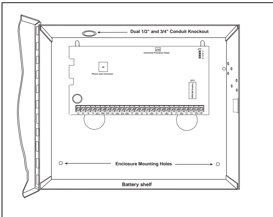
Figure 2: XR6/XR10/XR20 in standard enclosure
